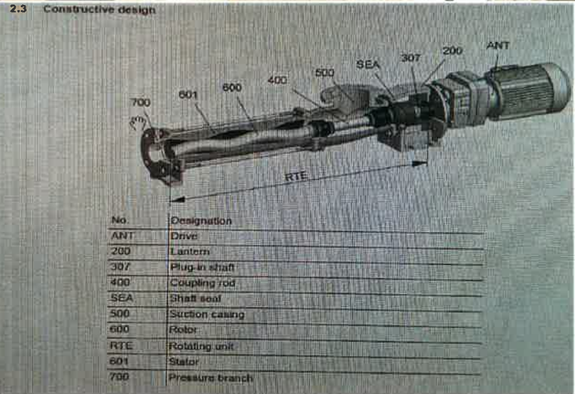
Grass Valley WWTP Primary sludge pumps re-build. The photo shows worn out “stators” due to the high volume of grit pumped by the primary sludge pumps during the 2019 storm events, along with the new stators (greased). The stator is shown on the diagram as Item # 601. Both the rotor and stators were replaced on both Primary sludge pumps post-2019 storm surge by the Mechanical Maintenance Department.
